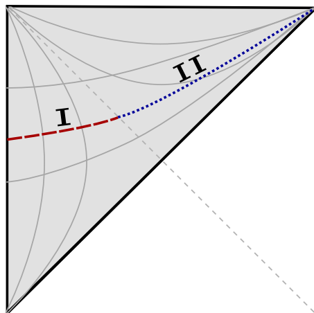
Figure 3: Penrose diagram for de Sitter space. Painlevé coordinates cover the shaded region. The curves are sections of constant t and constant r . Also shown is a constant-time slice split into two.
