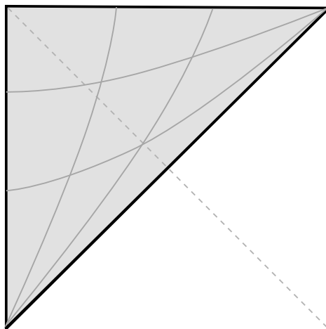
Figure 1: Penrose diagram for de Sitter space. Planar coordinates cover the shaded region. The curves are sections of constant \eta and constant \rho .
